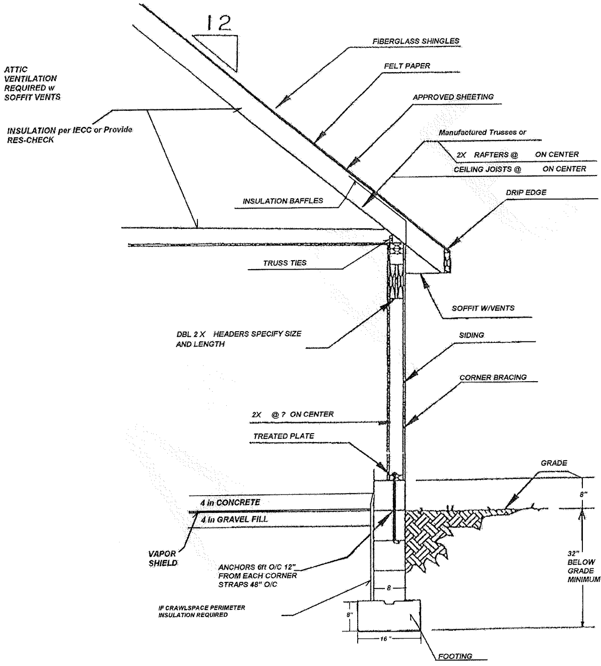
SECTIONAL VIEW
